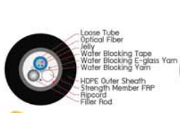
1 BELCOMMS MINI-3 TWISTED TUBE, ADSS 4-24 Core
