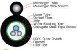
3 BELCOMMS MINI-3 TWISTED TUBE, Drop Wire 4-24 Core
