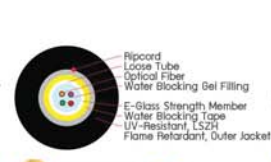
4 BELCOMMS Single Tube, ADSS 4-12 Core
