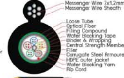
9 BELCOMMS Multi-Loose Tube, Messenger Wire 24-312 Cores
