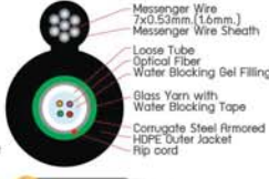
6 BELCOMMS Single Tube, Drop wire 4-12 Cores
